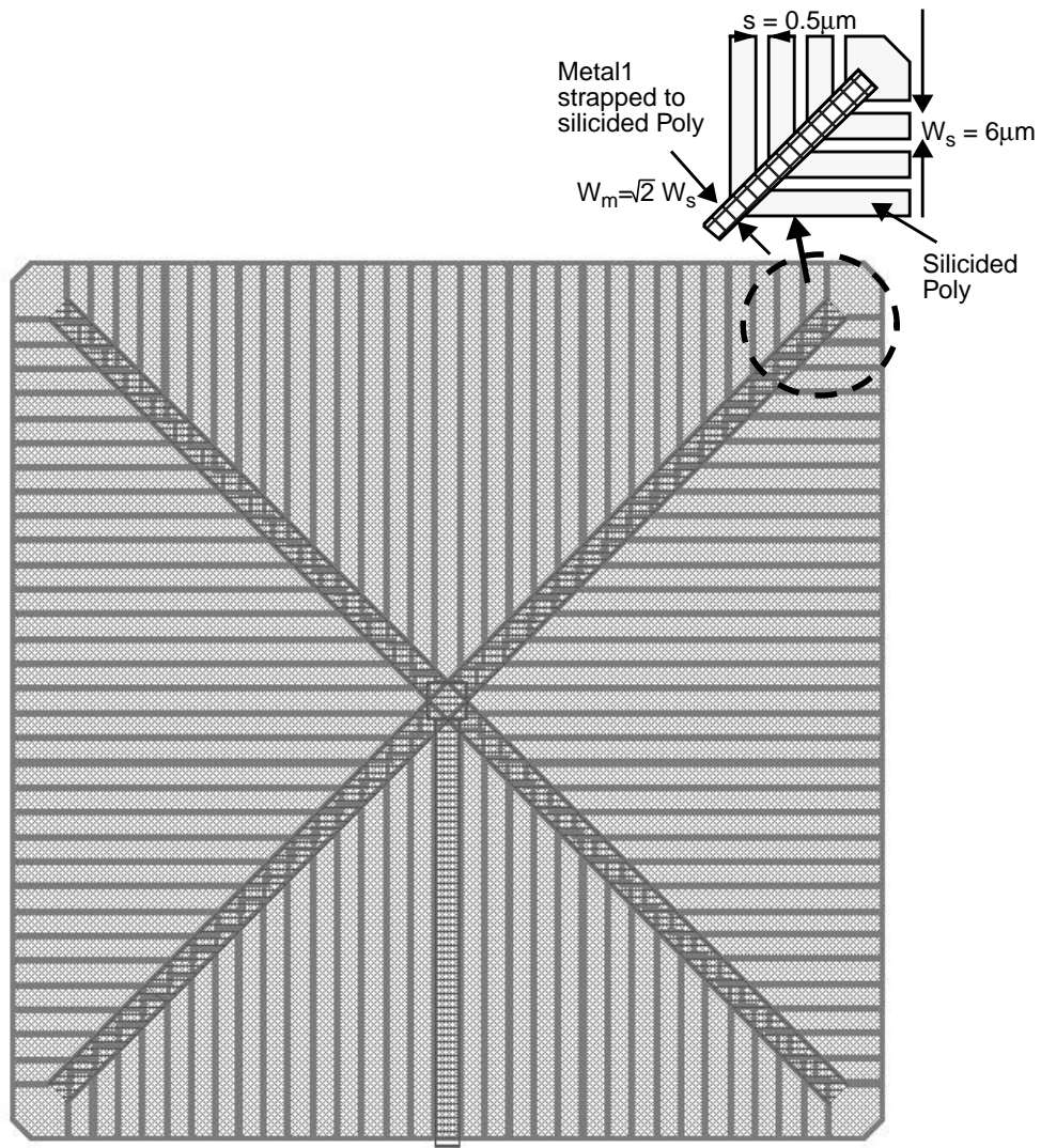
Top view for recommended PGS layout with polysilicon fingers and Metal-1 straps.
